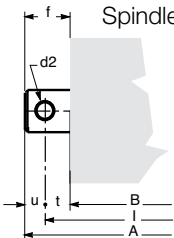
Spindle design K
