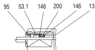
Straight Connector
