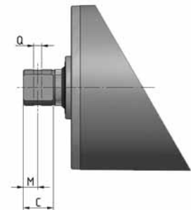
Shaft, cross-drilled and threaded.
